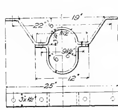
Figs. 4891-92. AXLE GUARD STRAP.
